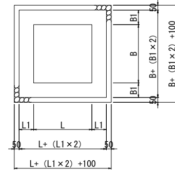
形 状 B L H B1 L1 h1 h2 足掛金具 摘 要 SM-B600-L600-H600 600 600 600 150 150 150 150 — SM-B700-L700-H600 700 700 600 150 150 150 150 — SM-B800-L800-H800 800 800 800 150 150 150 150 — SM-B800-L800-H900 800 800 900 150 150 150 150 — SM-B800-L800-H1200 800 800 1200 200 200 200 150 3 SM-B900-L900-H600 900 900 600 150 150 150 150 — SM-B900-L900-H700 900 900 700 150 150 150 150 —
